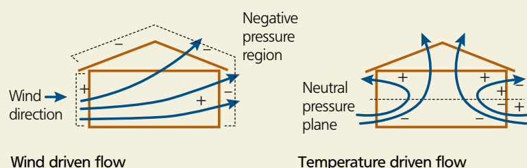
Figure 2 Schematic showing wind and temperature driven ventilation
